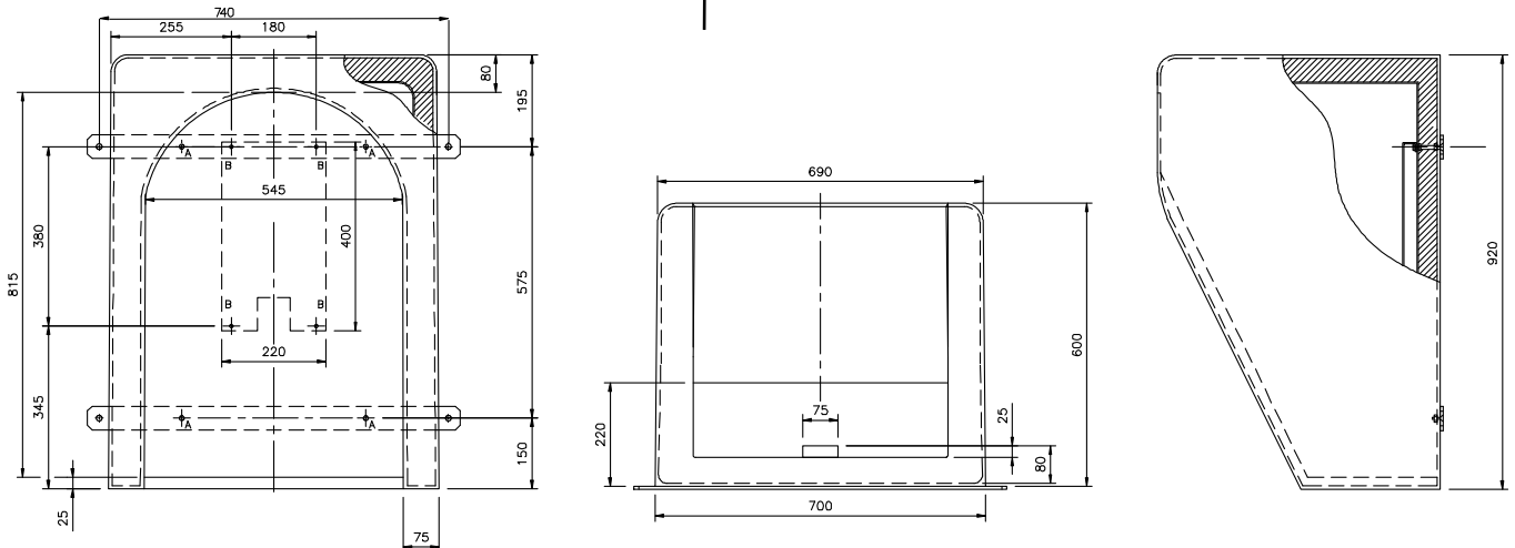
(Gear plate dimensions shown on this diagram are for 00*, 10* and 20* versions)
